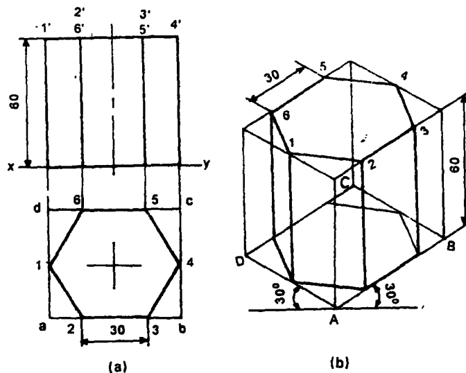
Fig. 9.19 Isometric Drawing of a Hexagonal Prism
