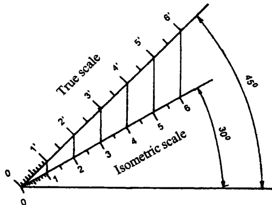
Fig. 9.3 Isometric Scale
