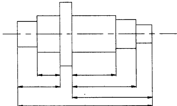
Fig. 2.35 Combined Dimensioning
