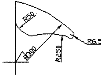
Fig. 2.24 Dimensioning of Radii
